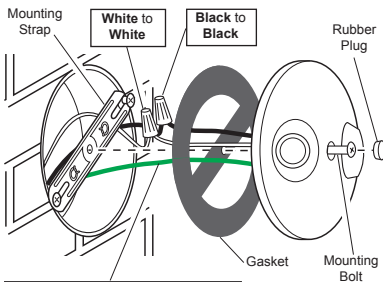
Wiring Floodlight
